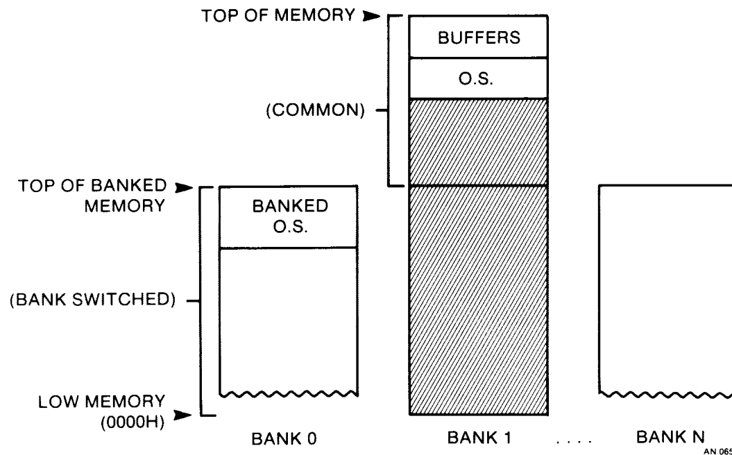
Figure 1-3. Banked Memory with Bank 1 in Context
