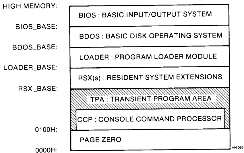
Figure 1-5. System Components and Regions in Logical Memory
