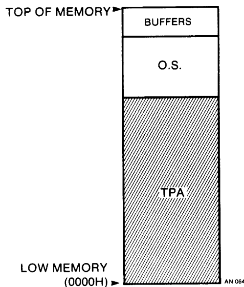
Figure 1-1. Nonbanked System Memory Organization
