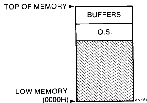
Figure 1-4. CP/M 3 Logical Memory Organization
