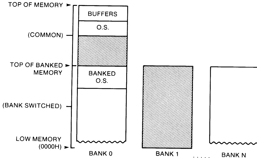
Figure 1-2. Banked System Memory Organization
