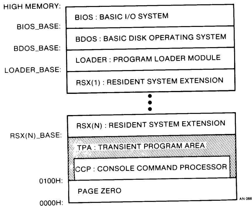
Figure 1-6. System Modules and Regions in Logical Memory
